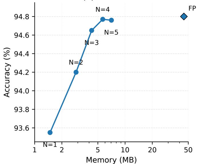
(b) ResNet-18
