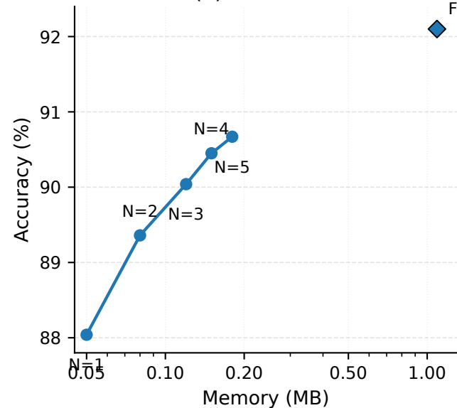
(a) ResNet-20
